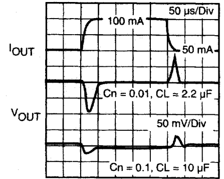
LOAD CURRENT STEP RESPONSE
