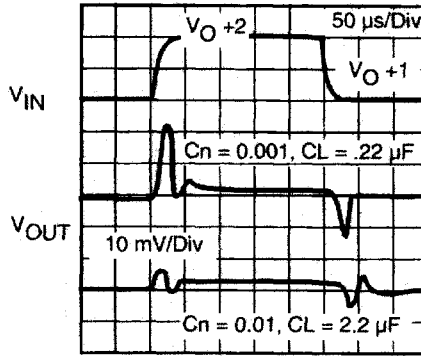
LINE VOLTAGE STEP RESPONSE
