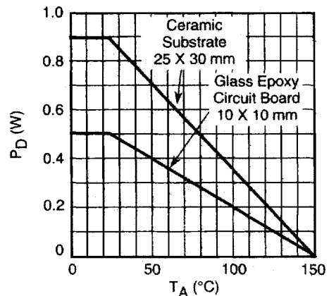
SOT-89-5 Power Dissipation Curve
