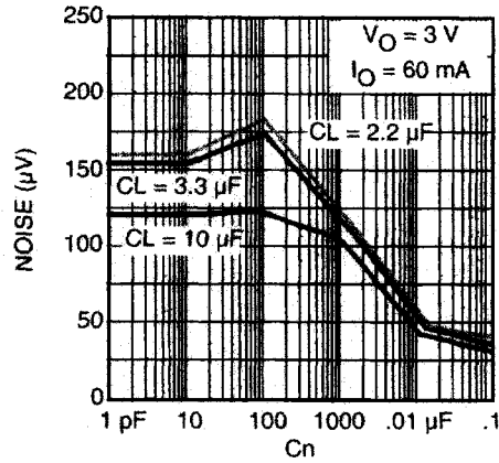
NOISE LEVEL vs. C_N
